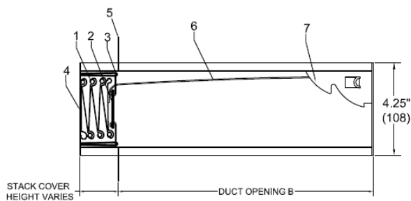
MODEL 51BHS-SS (HORIZONTAL MOUNT)
