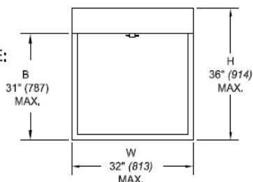
SINGLE SECTION DAMPER -HORIZONTAL MOUNT
