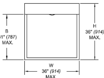
SINGLE SECTION DAMPER -HORIZONTAL MOUNT
